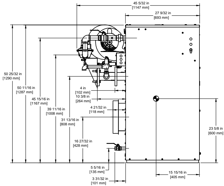
SIDE VIEW
